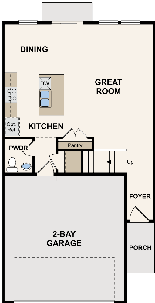
MAIN LEVEL
