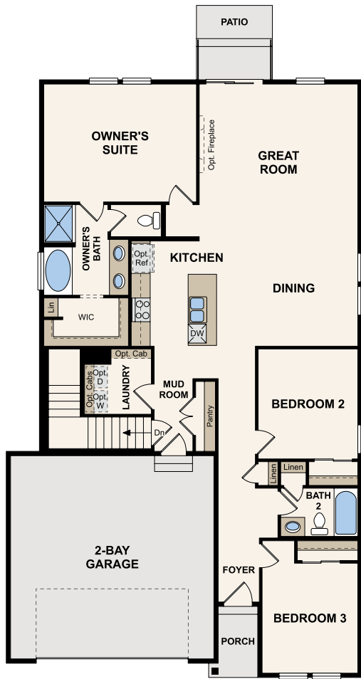
MAIN LEVEL
