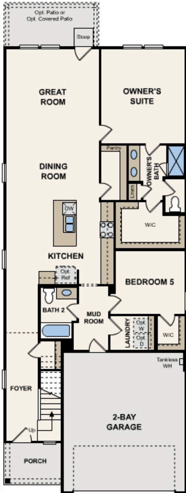
FIRST FLOOR
