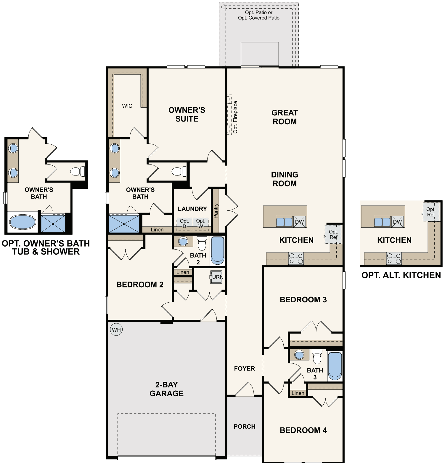
FLOOR PLAN
